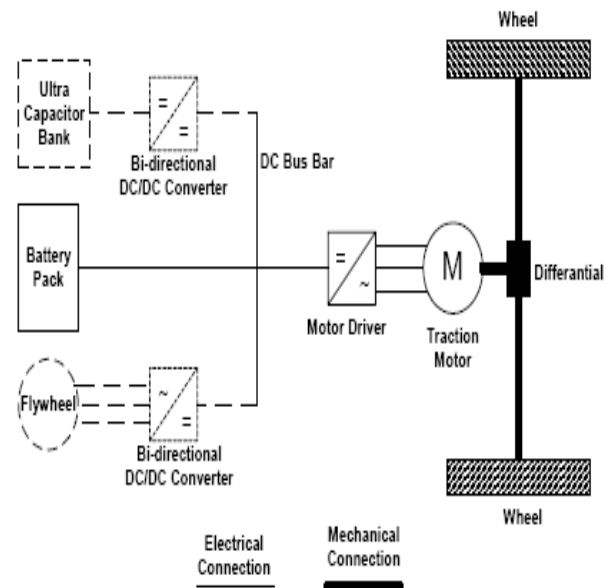
Figure 1. All Electric Vehicle Power train
