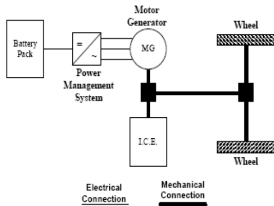
Figure 3. Parallel Hybrid Electric Vehicle Power train
