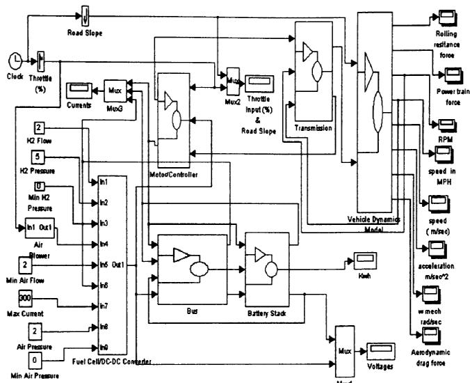
Figure 4. Simulink Model of a series HEV with Fuel Cell as the APU unit.
